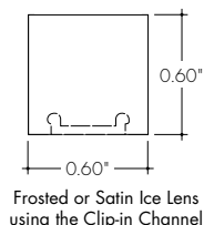
Fixture/Mounting Profile
