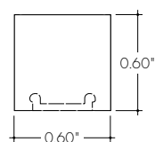
Frosted Lens using the Clip-in Channel
