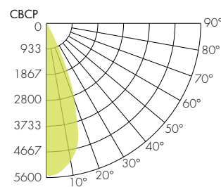
45° Smooth Reflector
