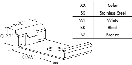
MB-KXLC-XX Fixed mounting clip -FC
