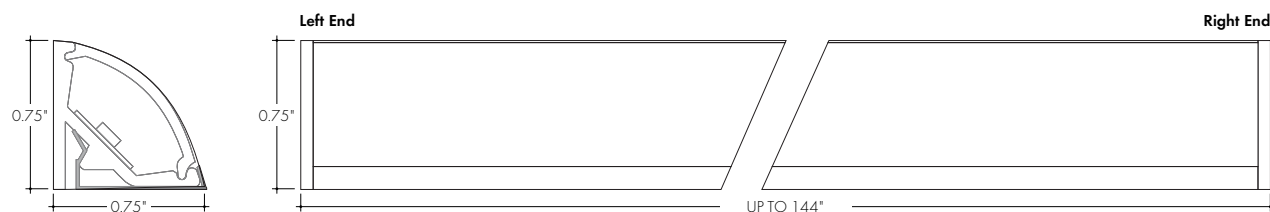
Front View (concealed mounting bracket on bottom)
