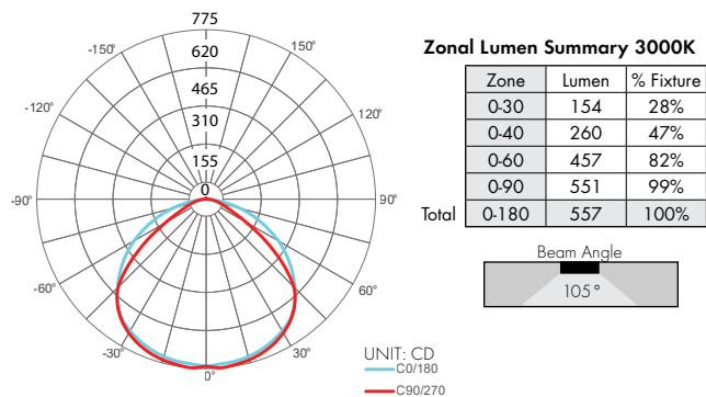
K45MW-48-VC72VHO-30K-C Kendo 45M Wet, 4ft, VHO, 3000K, Clear Lens
