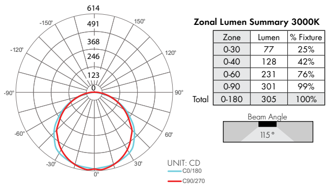
K45MW-48-VC72VHO-30K-F Kendo 45M Wet, 4ft, VHO, 3000K, Frosted Lens
