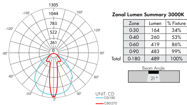
K45MW-48-VC72VHO-30K-13 Kendo 45M Wet, 4ft, VHO, 3000K, 13° Semi-Frosted
