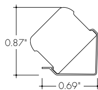
Narrow Beam Grazer Lens with 45° Mounting Bracket
