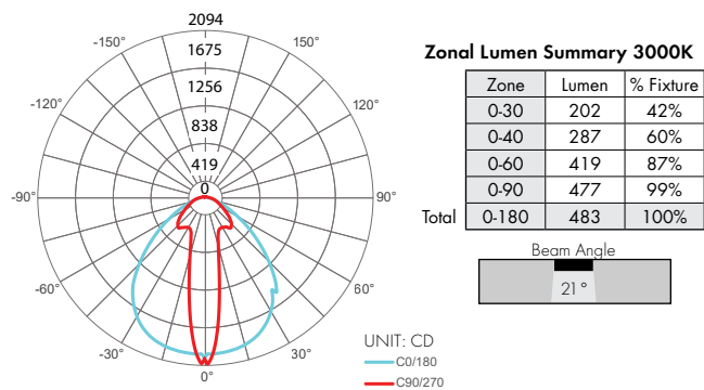
KMW-48-VC72VHO-30K-GR
