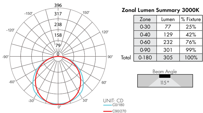
KMW-48-VC72VHO-30K-F
