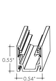
KBS Mounting Channel, Serrated Aluminum Profile
