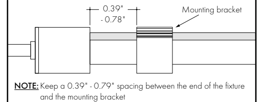
KBL 3-Side Emitting Mounting Channel, Serrated Aluminum Profile
