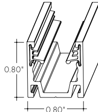
KBL Mounting Channel, Serrated Aluminum Profile
