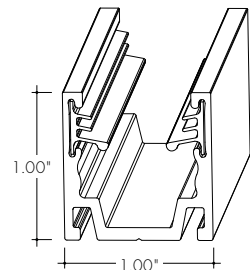
KBX Mounting Channel, Serrated Aluminum Profile
