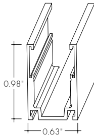
KBM Mounting Channel, Serrated Aluminum Profile
