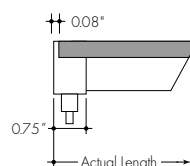
Back Connector -IMB
