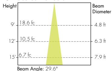
30° Faceted Reflector
