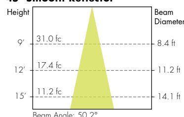
45° Smooth Reflector
