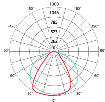
MK45-48-VC72VHO-30K-F
