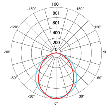
MK45-48-VC72VHO-30K-MF
