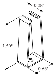
Catenary Mount, Decorative Clip
