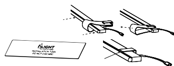
Mounting Clip Installation Tool
