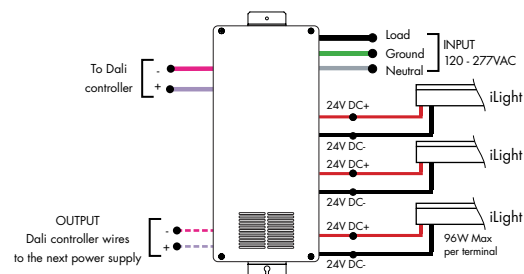
PS-DALI-D-3X96-24
