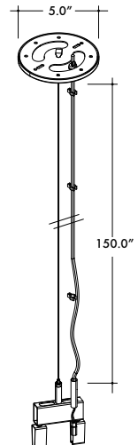
SC-1FC5-DCL-C2-0X-0Y Powerfeed Canopy Suspension Kit with Joiner Clip, Ø5.0" canopy, 150" A/C Cable
