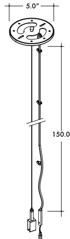
SC-1FC5-SCL-C2-0X-0Y Powerfeed Canopy Suspension Kit with Single Clip, Ø5.0" canopy, 150" A/C Cable
