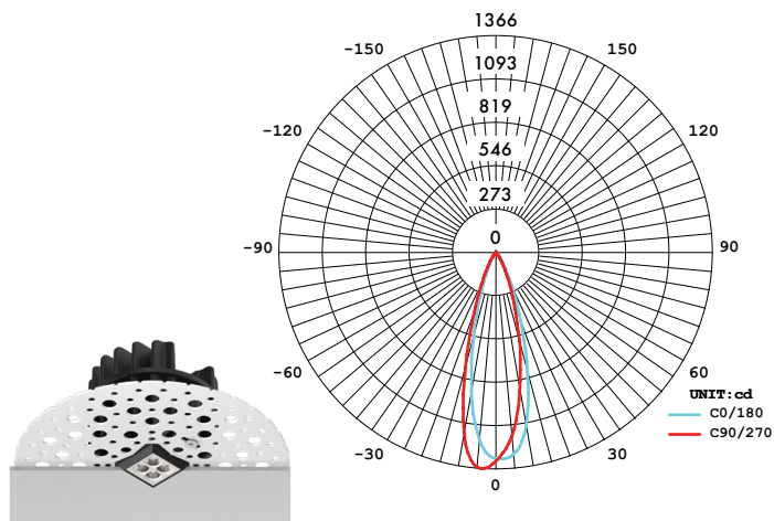
30° Optic and Louver
