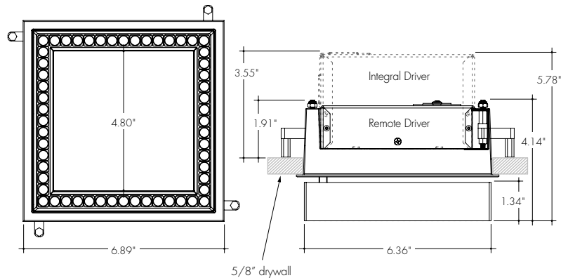
Stenos Square 6" Recessed Adjustable Downlight
