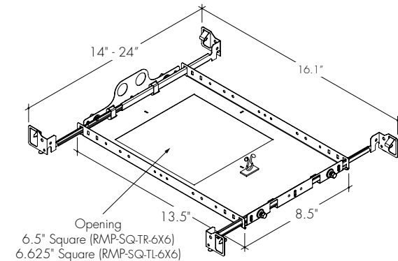
RMP-SQ-TR-6X6 / RMP-SQ-TL-6X6 6" Recessed New Construction Mounting Pan
