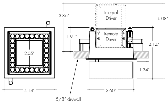
Stenos Square 4" Recessed Adjustable Downlight
