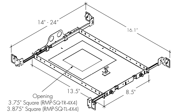
RMP-SQ-TR-4X4 / RMP-SQ-TL-4X4 4" Recessed New Construction Mounting Pan
